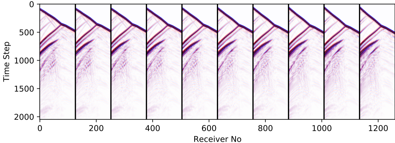
vModel-10-test-shot-50-59-vz
