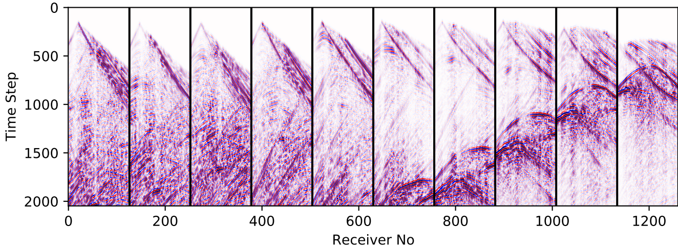
vModel-80-train-shot-50-59-curl
