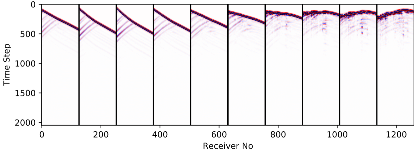
vModel-52-train-shot-50-59-div
