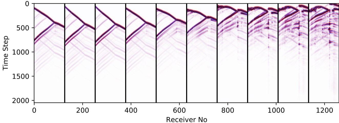
vModel-453-train-shot-50-59-div
