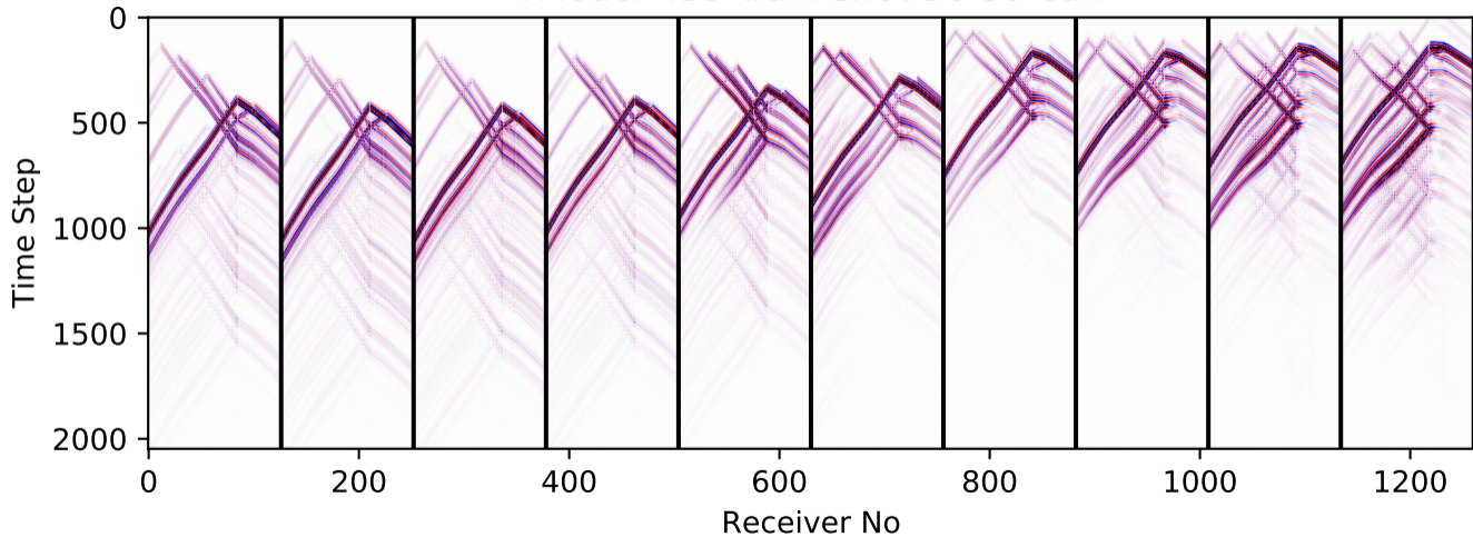
vModel-453-train-shot-50-59-curl
