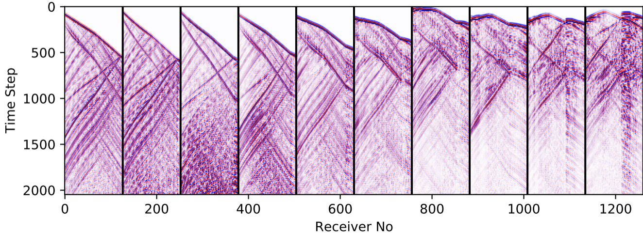
vModel-452-train-shot-50-59-vx
