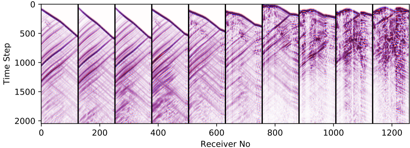
vModel-452-train-shot-50-59-div
