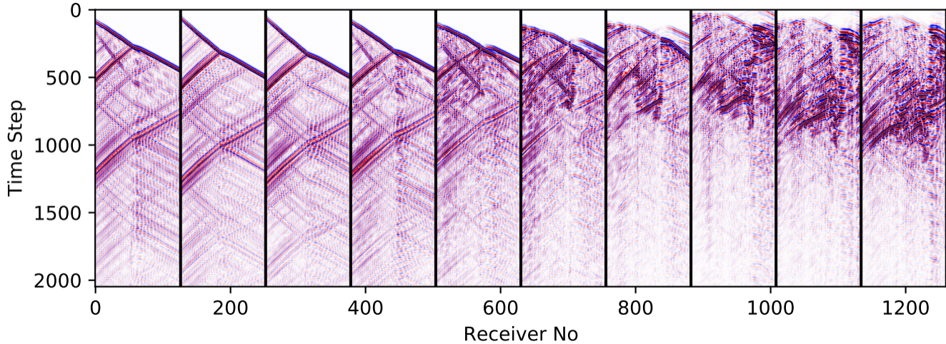
vModel-451-train-shot-50-59-vz
