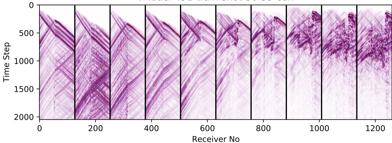
vModel-451-train-shot-50-59-curl
