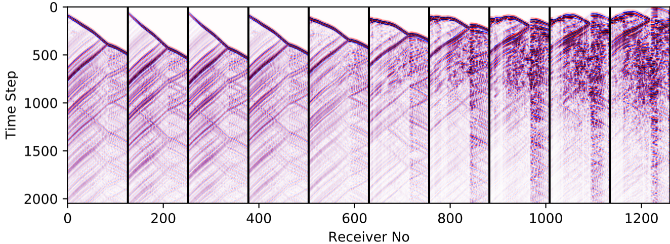
vModel-450-train-shot-50-59-div
