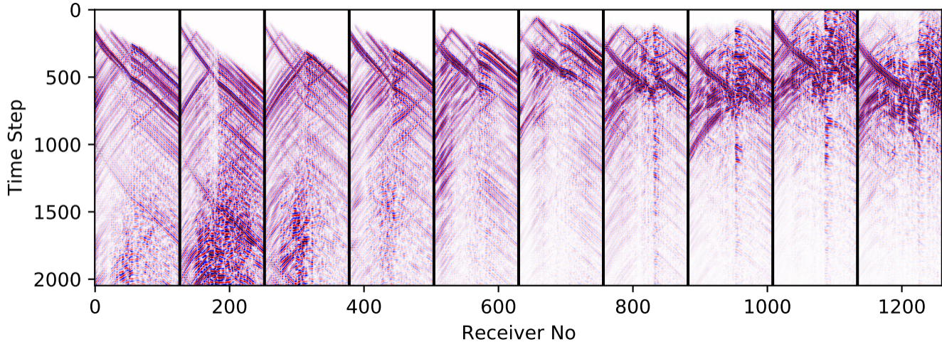
vModel-431-train-shot-50-59-curl
