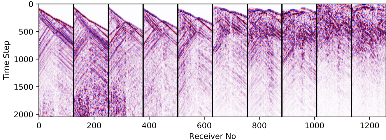
vModel-430-train-shot-50-59-vx
