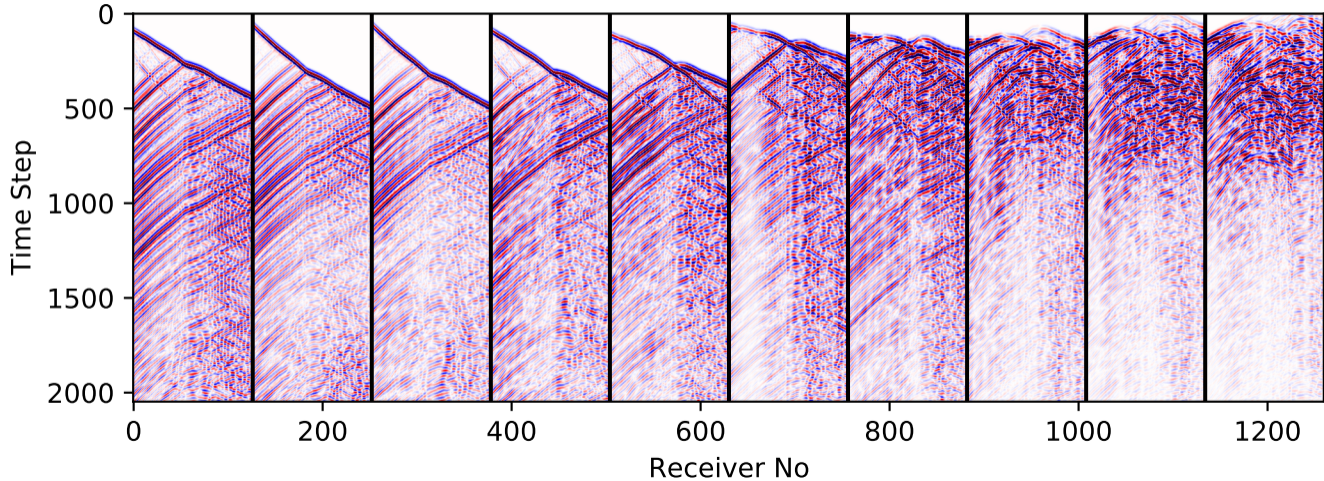
vModel-419-train-shot-50-59-vz
