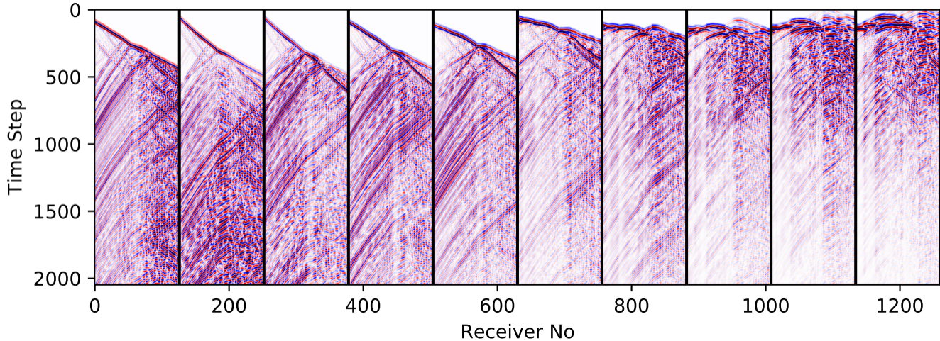
vModel-419-train-shot-50-59-vx
