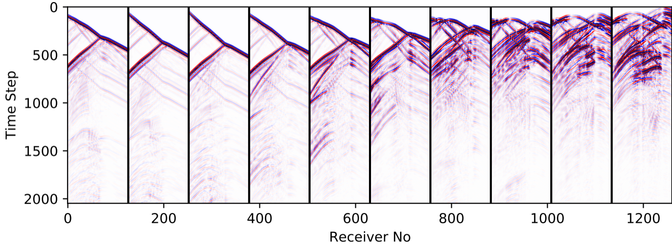
vModel-10-train-shot-50-59-vz
