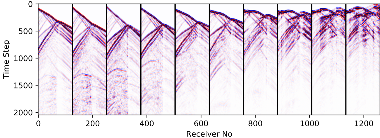
vModel-10-train-shot-50-59-vx
