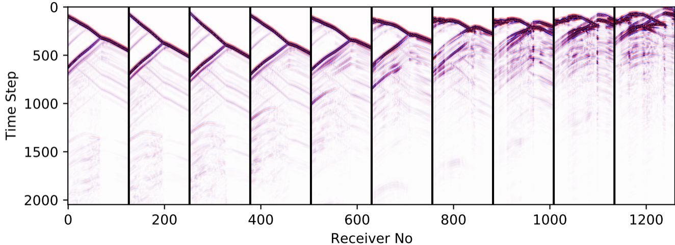
vModel-10-train-shot-50-59-div
